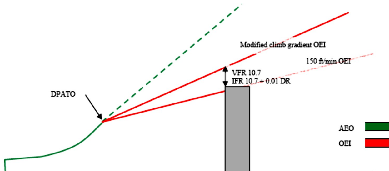
Figure 6: Performance Class 2 (enhanced climb gradient)
