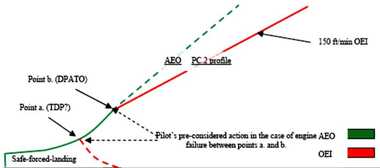
Figure 5: The three elements in a PC 2 take-off
