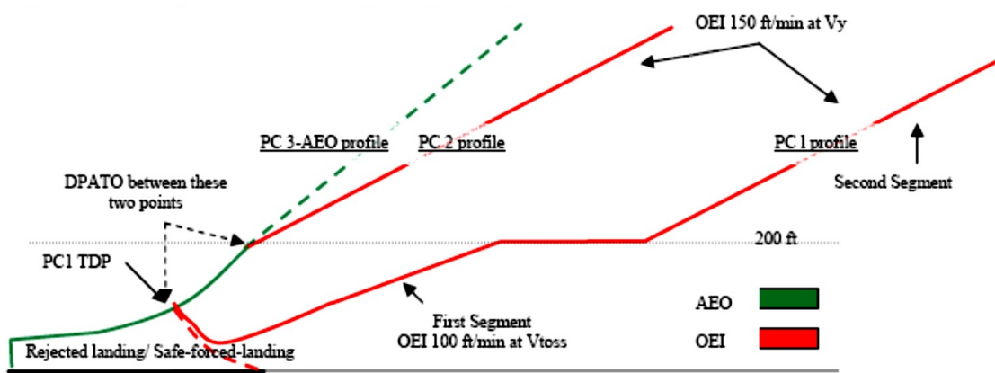
Figure 1: All Performance Classes (a comparison)
