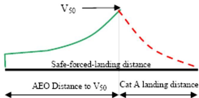
Figure 10: Category B ( V_{50} ) safe-forced-landing distance
