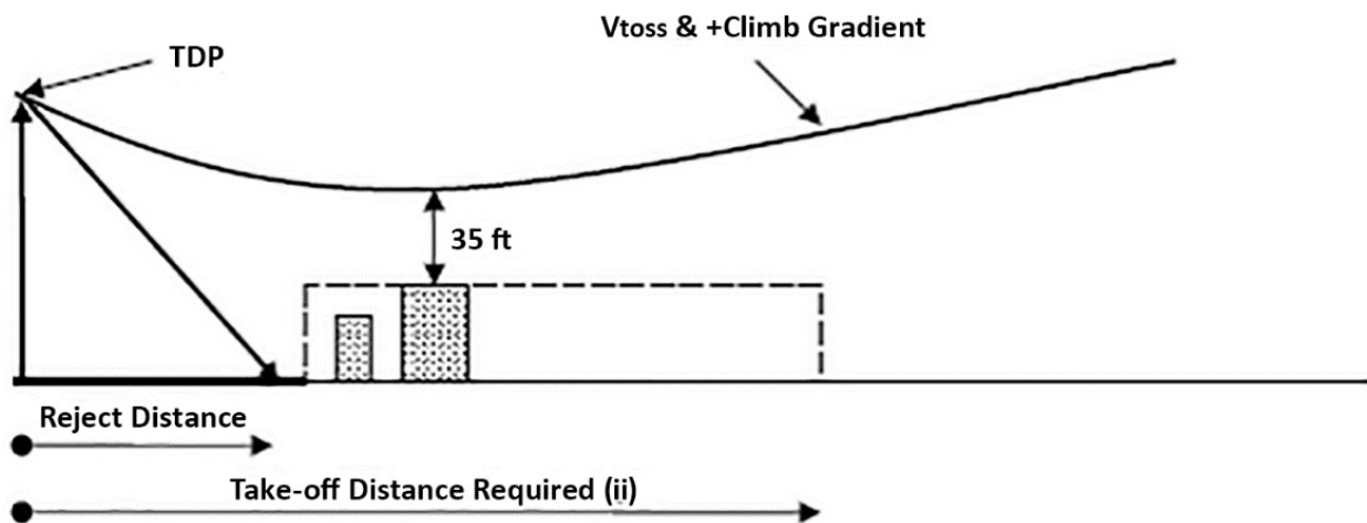
Figure 2 Short Field take-off
